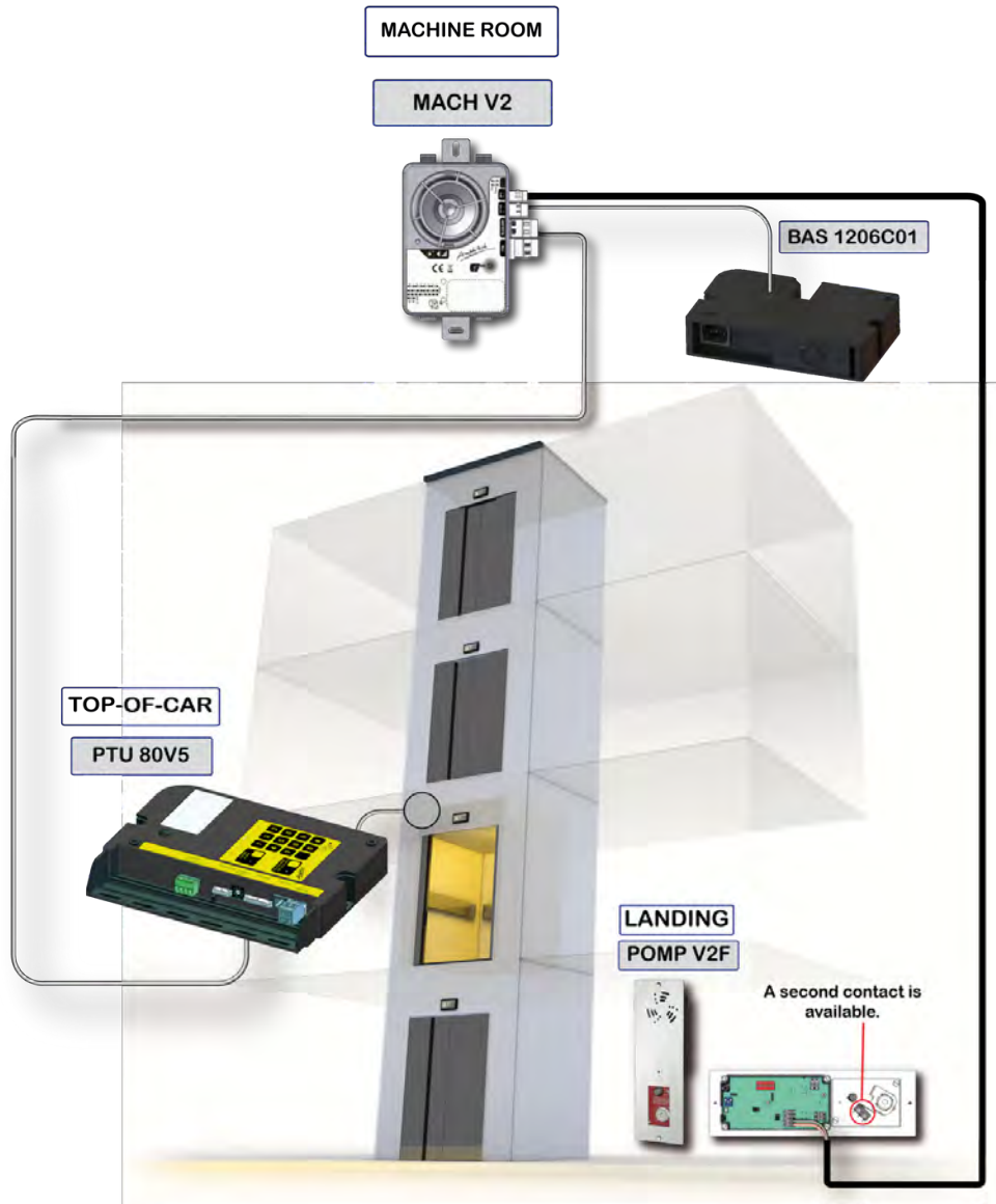
Figure 1. Wiring
